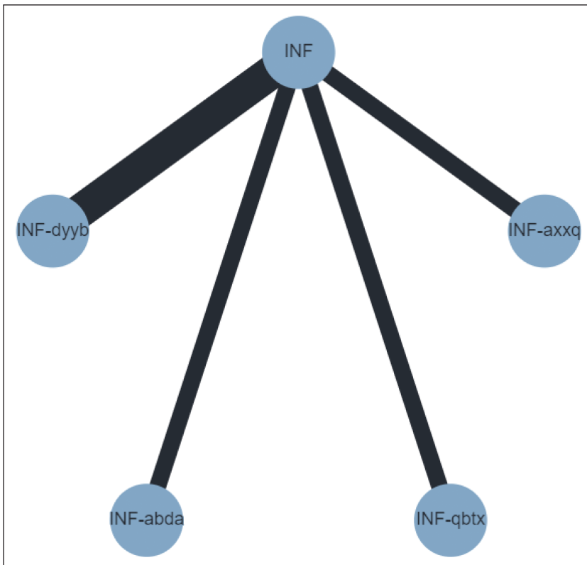
Figure 2. Network diagram of included articles. Each node represents one treatment, while lines show direct comparisons in the included studies; line thicknesses is proportional to the number of studies with these comparisons.
